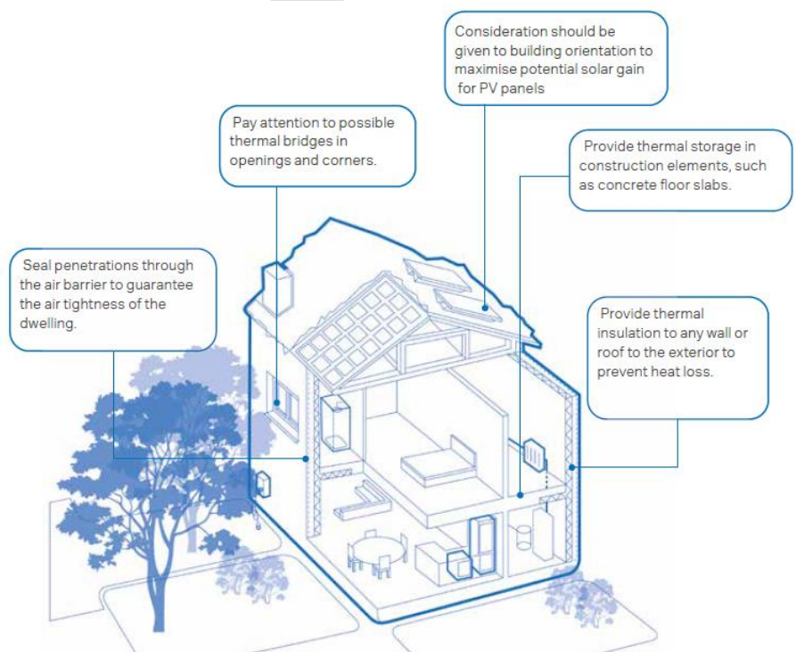
Figure: 17 Diagram illustrating aspects relevant to energy efficient designs
